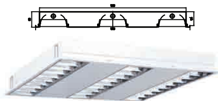
Two central solid/perforated sheet metal strips
